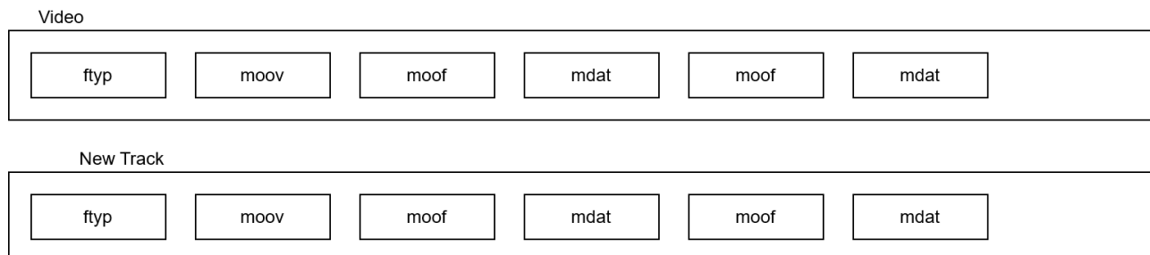
Diagram 7: CMAF late binding:
