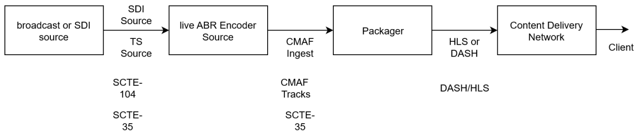
Diagram 9: Example setup schema with CMAF ingest and DASH/HLS ingest
